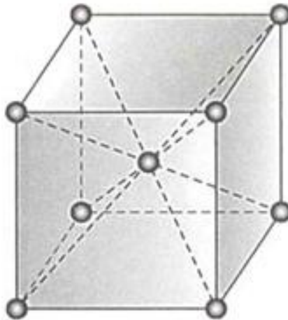
bcc
