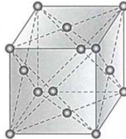
fcc
