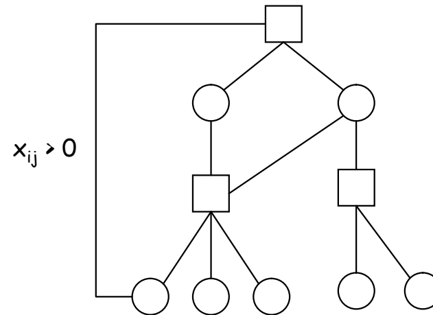
G(x) cyclic
