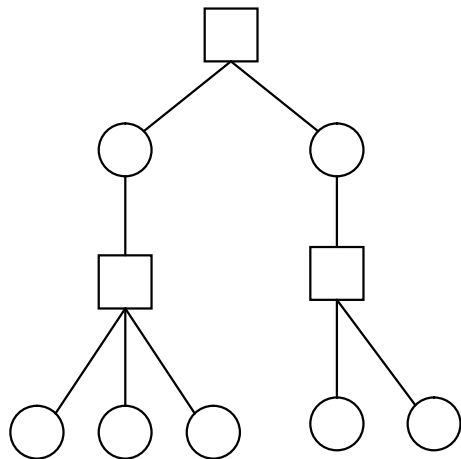
G(x) acyclic
