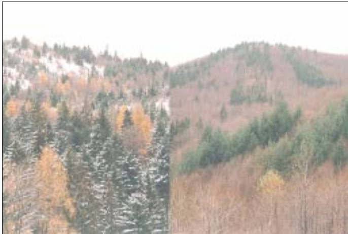
Fig. 70 Representative demonstration of the quoted class on examples of mixed forest (created by alternation of single trees and stands of trees) in Stiavnické vrchy (Slovakia)
