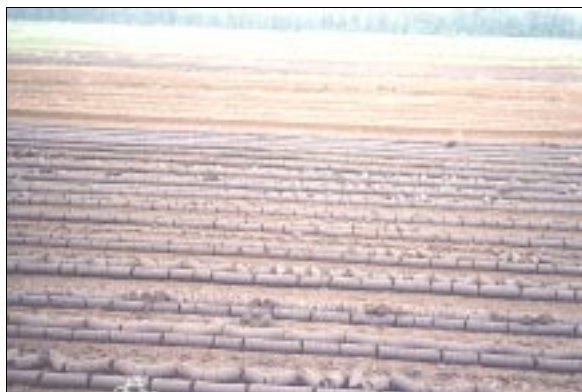
Fig. 106 Representative of the quoted class particularity on example of the exploited peat bog in Lithuania
