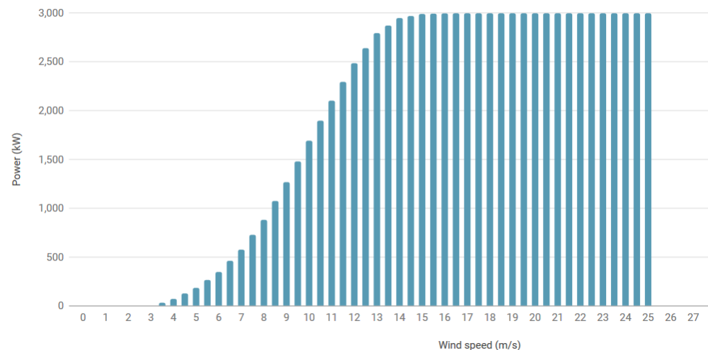
Power curve
