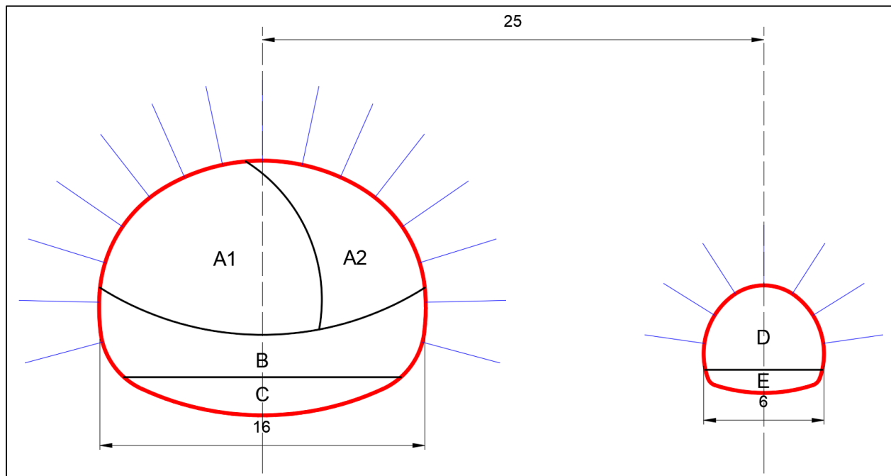
Figure 1. Tunnels section.
