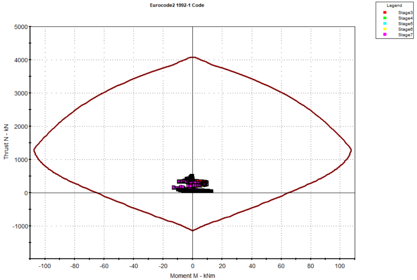
Figure 6. Support capacity plot for the composite lining of shotcrete and steel sets.
