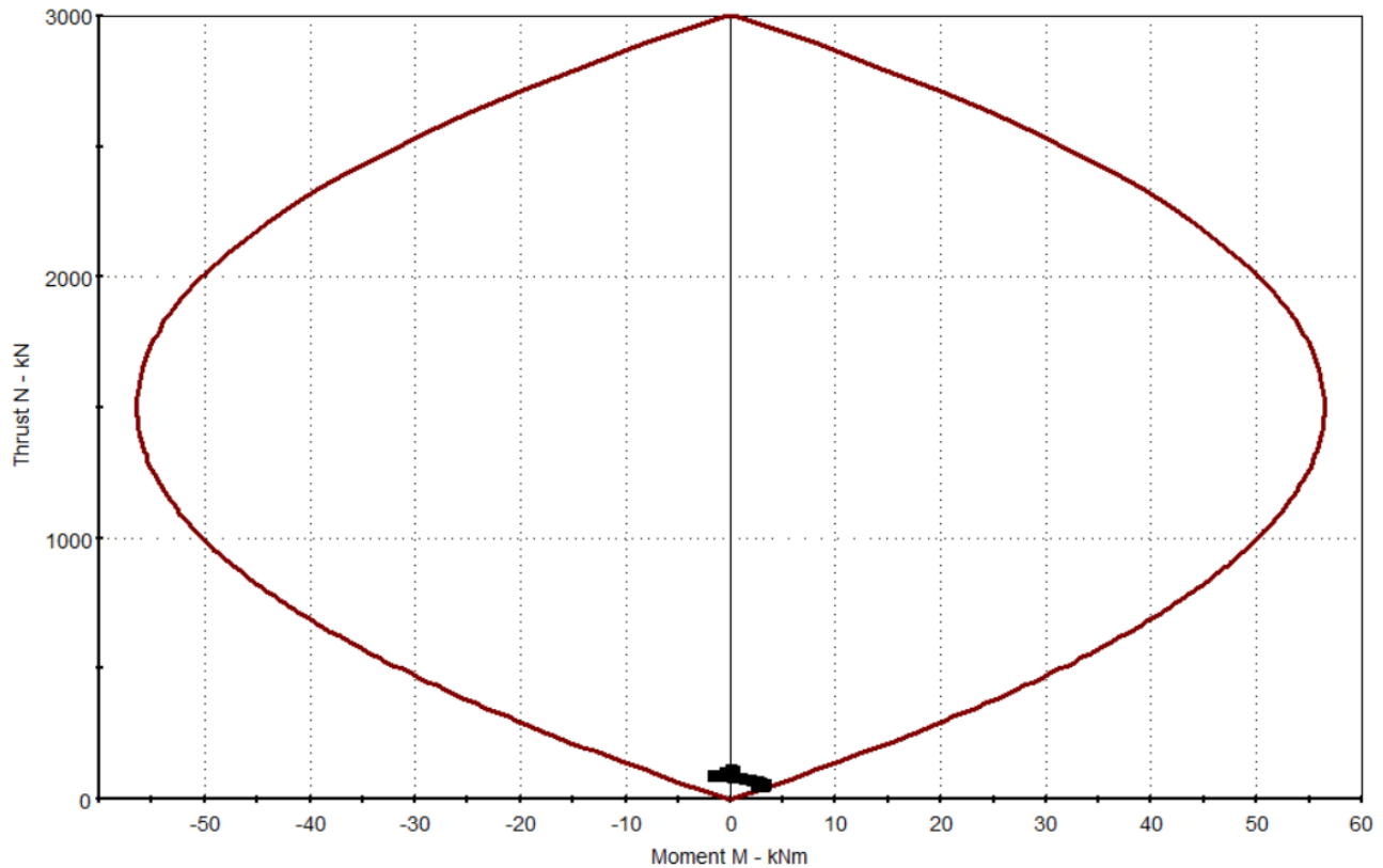
Figure 7. Support capacity plot for the tunnel invert lining.
