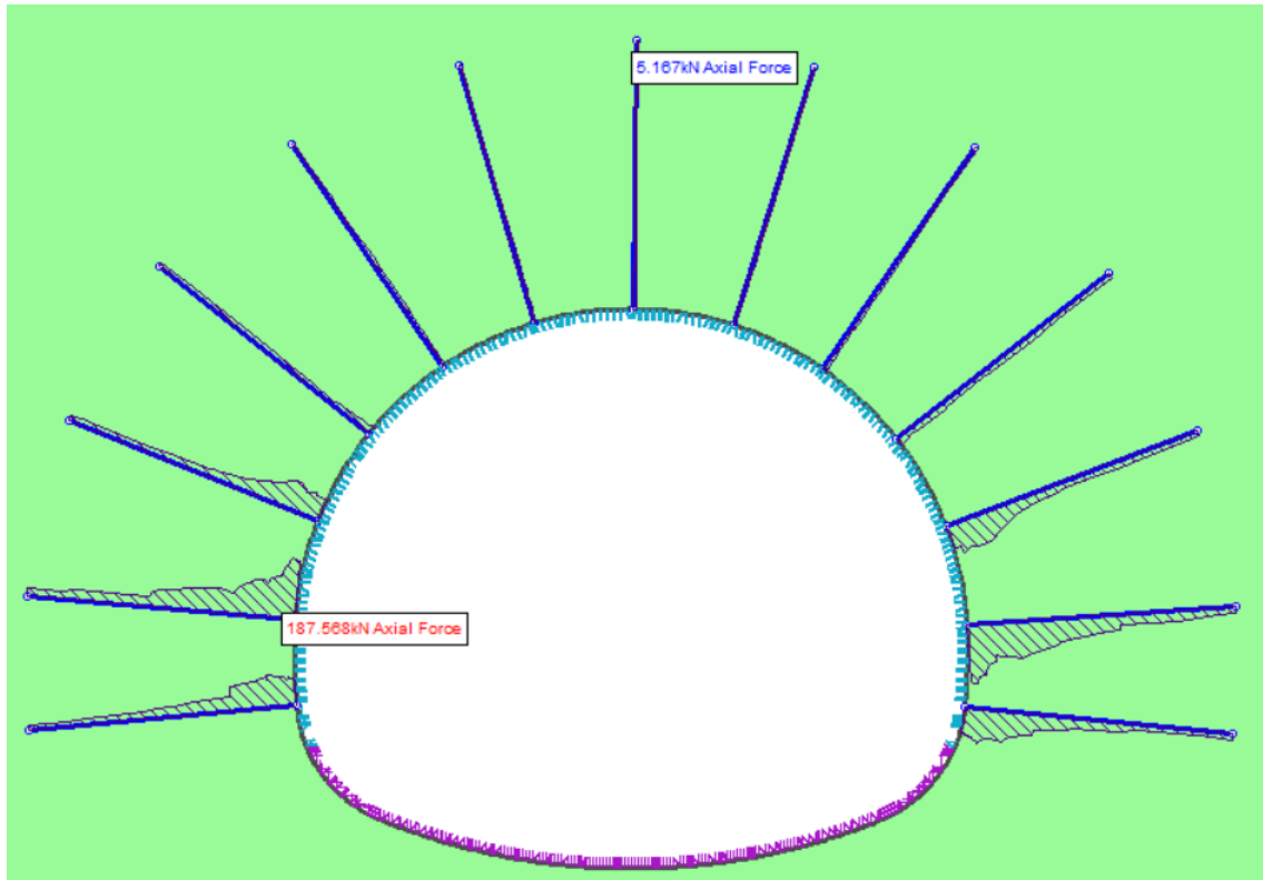
Figure 8. Axial force on tunnel perimeter rockbolts.
