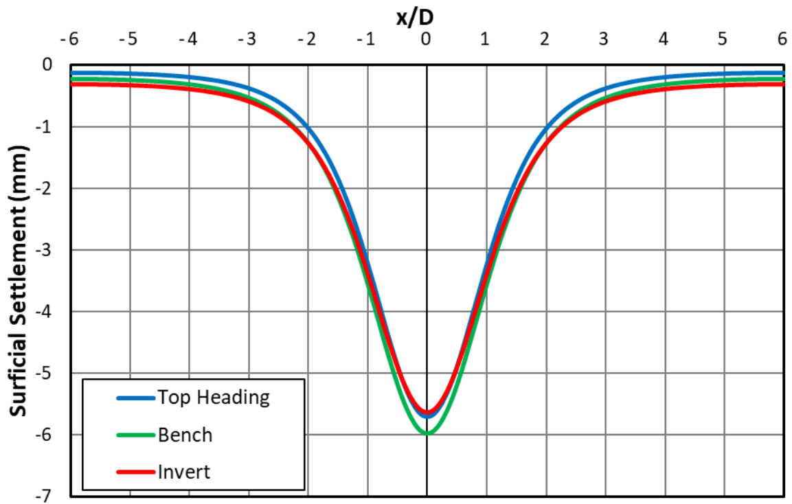
Figure 9. Surficial settlement profile.
