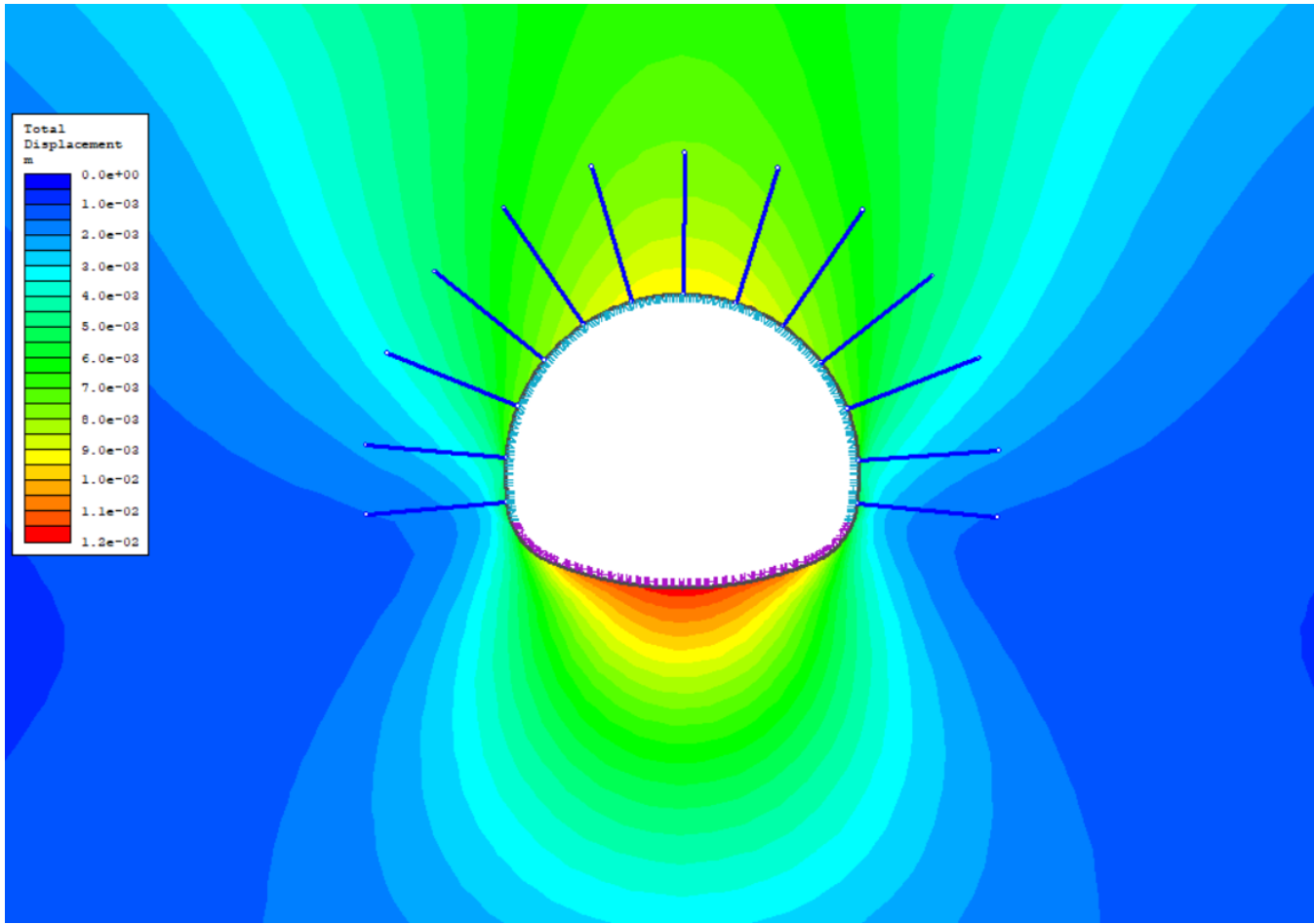
Figure 10. Total displacements on the final excavation stage.
