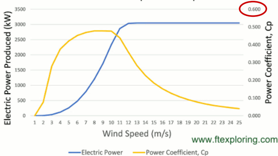
Electric Power & Cp vs. Wind Speed
