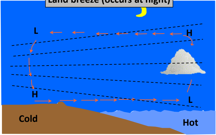
Land breeze (occurs at night)
