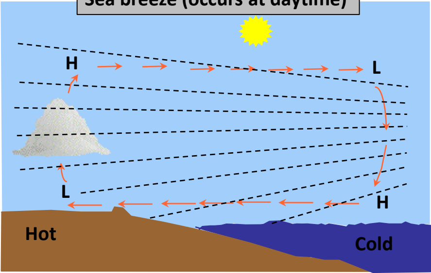
Sea breeze (occurs at daytime)
