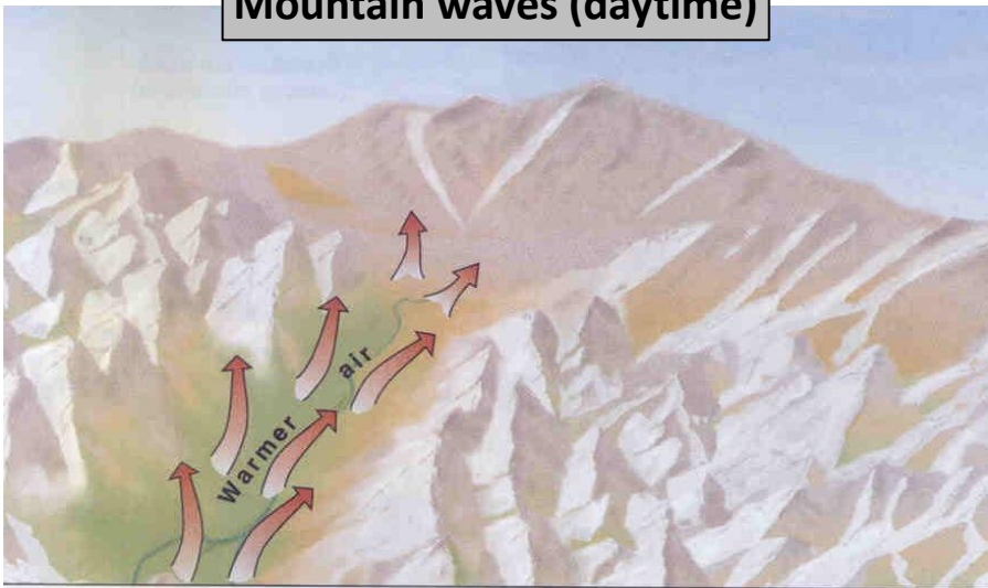
Mountain waves (daytime)
