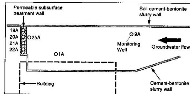
Figure 4 - Plan view, treatment wall and slurry wall system.
