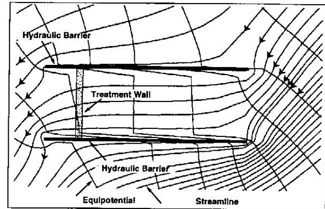
Figure 3 - Groundwater flow modeling of treatment wall and slurry wall system.
