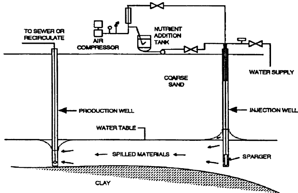
Fig. 1. Typical system.
