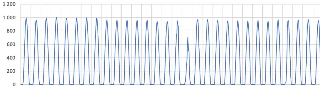
Mean hourly solar radiation data at Aktion (July 2017)
